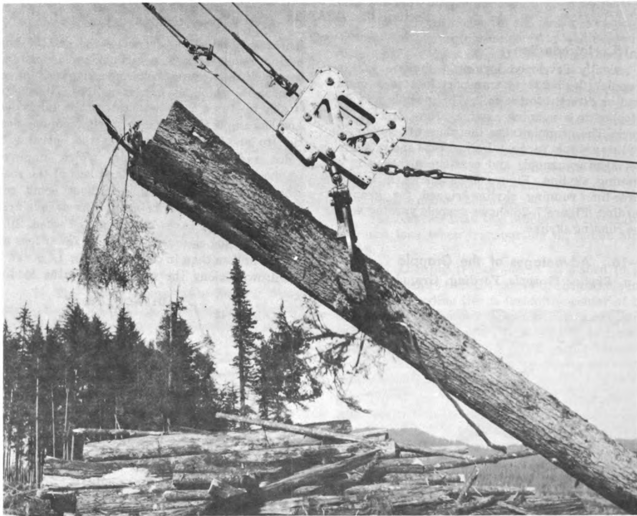
Figure 7-26. Grapple yarding with running skyline.
